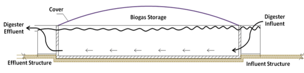
Figure 3.8. Plug-flow Digester Diagram 26
