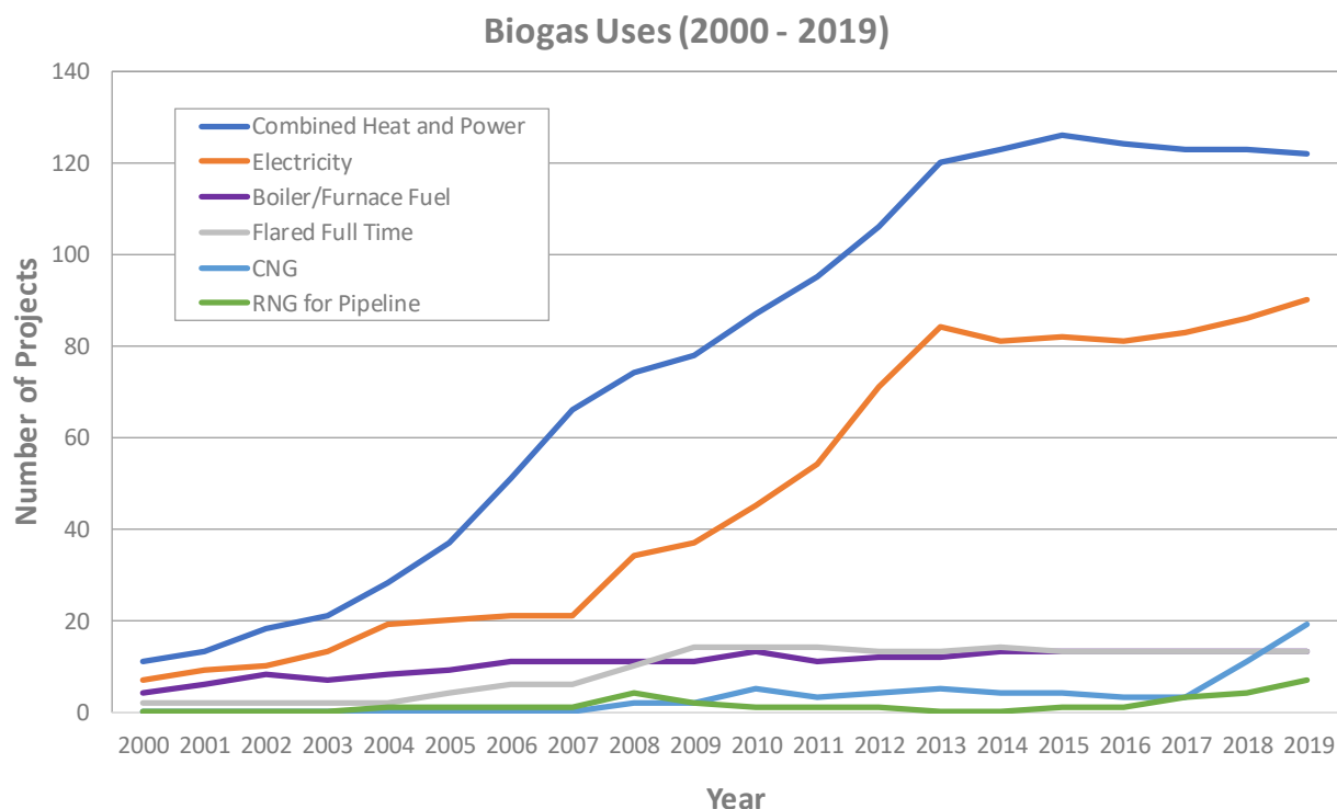
Figure 5.1. Biogas End Uses at Farms 40
